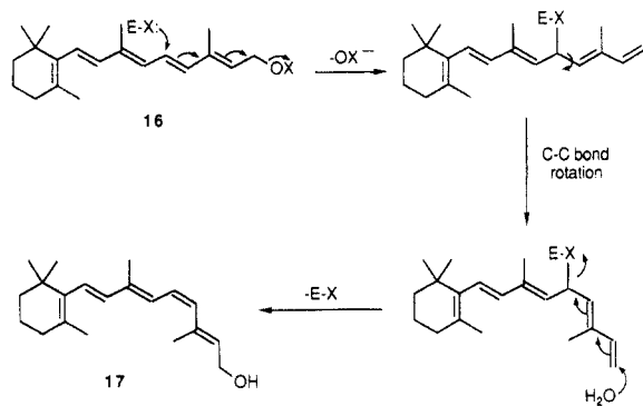
Figure 16. Biological precedent for double- S_N2' reaction.
