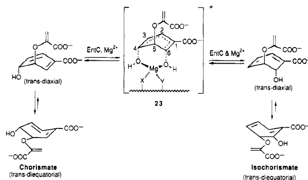
Figure 20. Concerted 1,5 double- S_N2' displacement mechanism.
