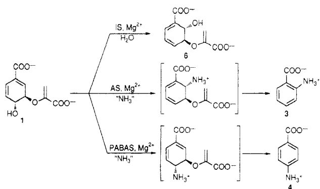
Figure 9. Comparison of isochorismate synthase with anthranilate synthase and PABA synthase.
