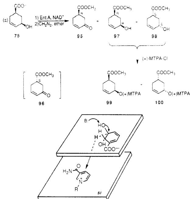
Figure 28. Schematic of the active site of the Ent A protein. From the mechanistic studies, the C 3 proton is stereospecifically removed as a hydride and transferred to the si face of NAD + .
