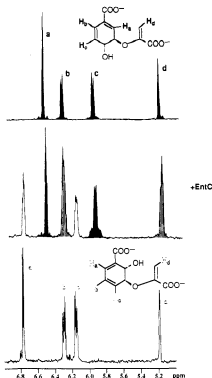
Figure 12. 1 H NMR spectra of chorismate (top), isochorismate (bottom), and an equilibrium mixture of both in the presence of isochorismate synthase (middle).
